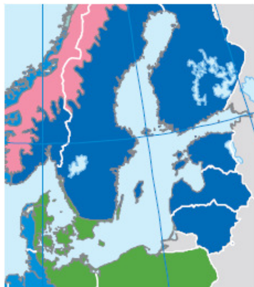
Fig. 1. Projected impacts of climate change in Baltic Sea countries as European regions
