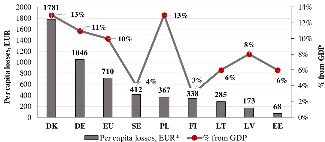
Fig. 2. Impacts of extreme weather and climate related events in Baltic Sea countries, 1980-2017
